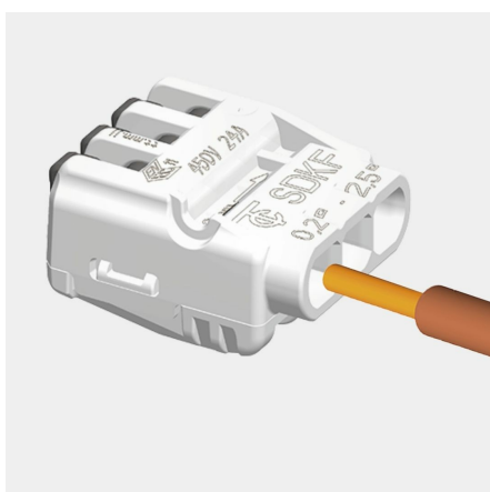
For solid wires it is not necessary to open the lever before pushing in the wire
